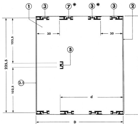
6U x 84HP Type 2 & Type 3 MOTHERBOARD
